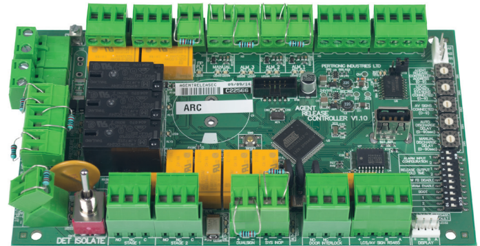
Extinguishing Agent Release Controller
