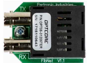
Fibre-optic converters for the Pertronic Net2 Card with ST connectors (above) and SC connectors (below)
