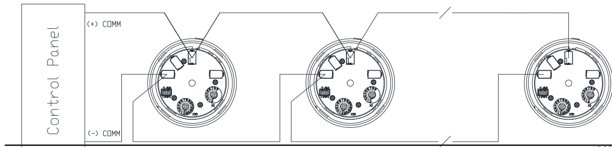
Figure 5 System wiring diagram
